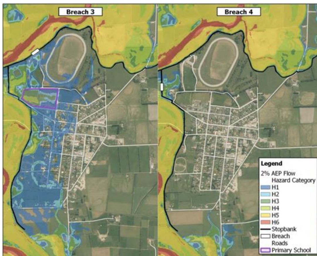
Figure 6 – Hazard maps for breach 3 and 4.
