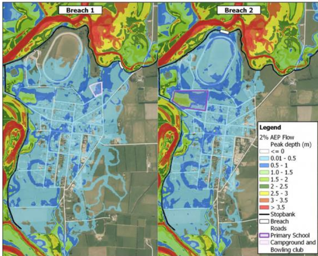
Figure 5 – Peak depth for the 2% AEP breach 1 and 2 scenarios.
